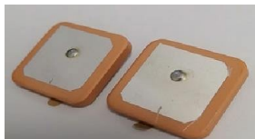
P/N: VEDYS35N4 Name: Ceramic Antenna Freq: 1575.42-1610MHz Dim: 35×35×4mm
